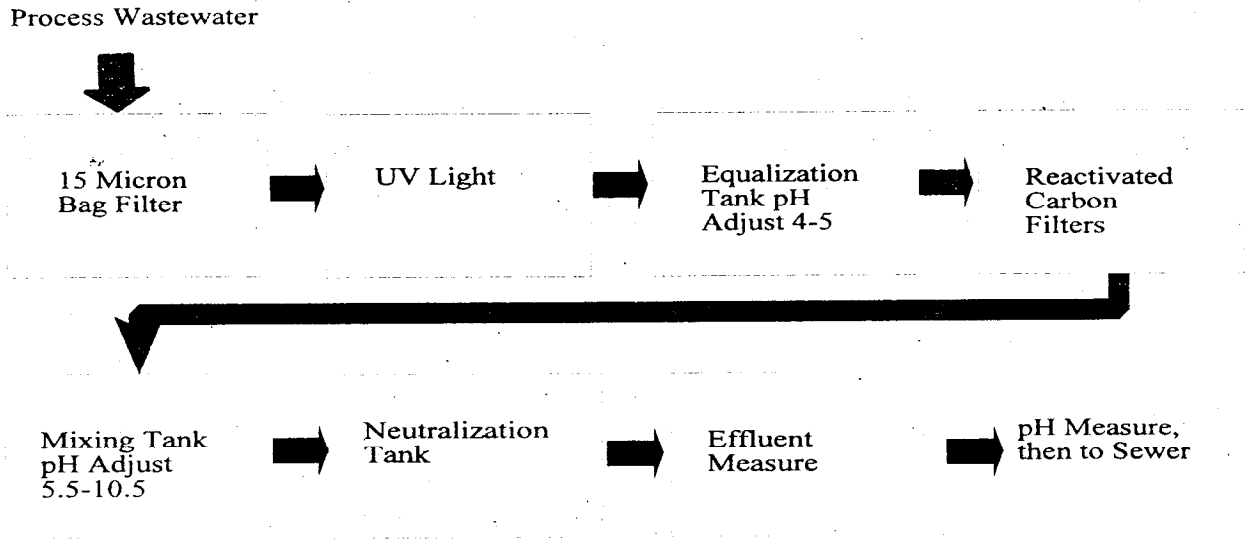
Figure 1: Schematic of Wastewater Treatment System
