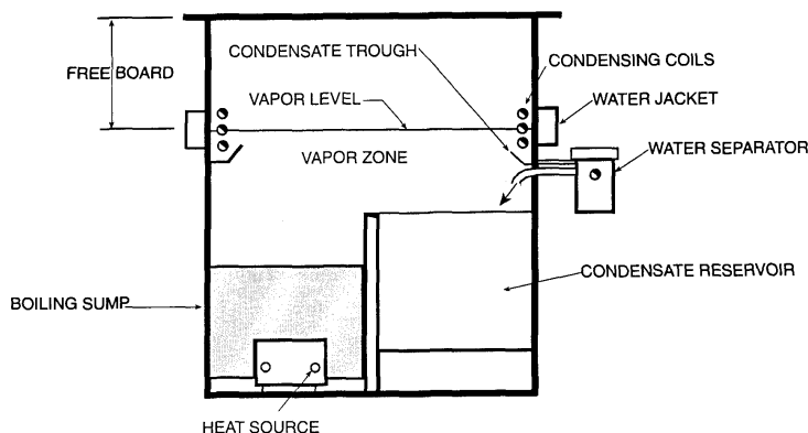
Figure 1 - Open Top Vapor Degreaser
