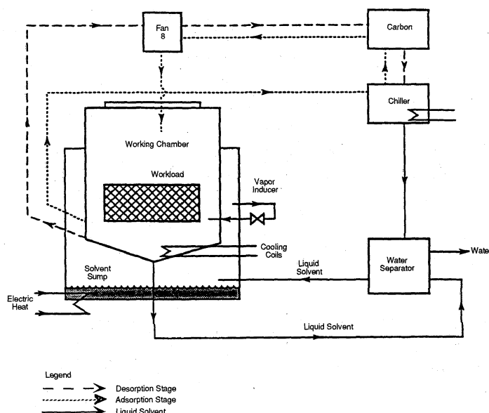
Figure 2 - Closed-Loop Vapor Degreaser (Source: U.S. EPA, Guide to Cleaner Technologies, Cleaning and Degreasing Process Changes , EPA/625/R-93/017, February 1994)
